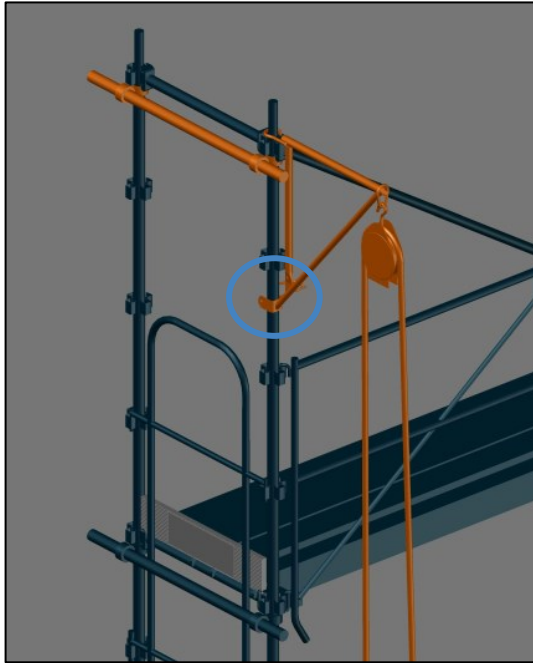
Figure 73 : Cas 1 => Position fixe
