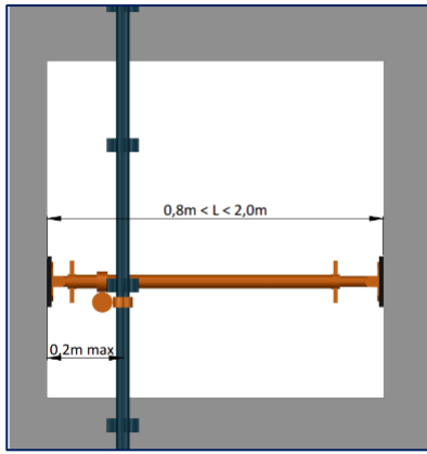
Figure 53: Véringage (vue de face)
