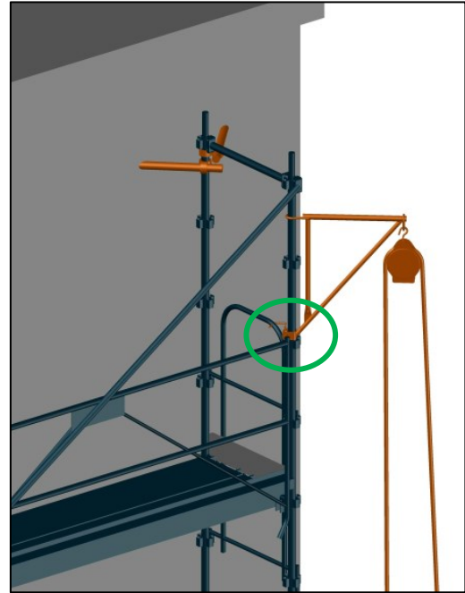
Figure 74: Cas 2 => Position rotative
