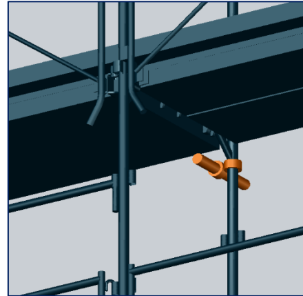
Figure 40 : Amarrage simple
