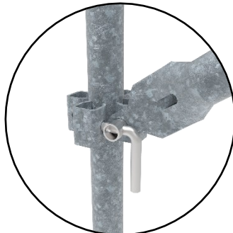
Figure 25 : Assemblage diagonale DV
